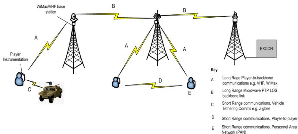
Figure 4-2: TES Infrastructure.
