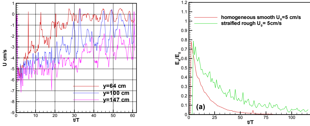
Figure 2: (a) The average kinetic energy for the impulsively started downwelling favorable flow over continuous topography. (b) Along-shelf velocity component obtained at the shelf-break level for the no-canyon case.
