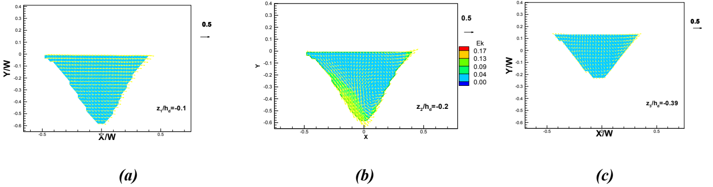
Figure 3: Normalized kinetic energy distribution for the smooth canyon.
