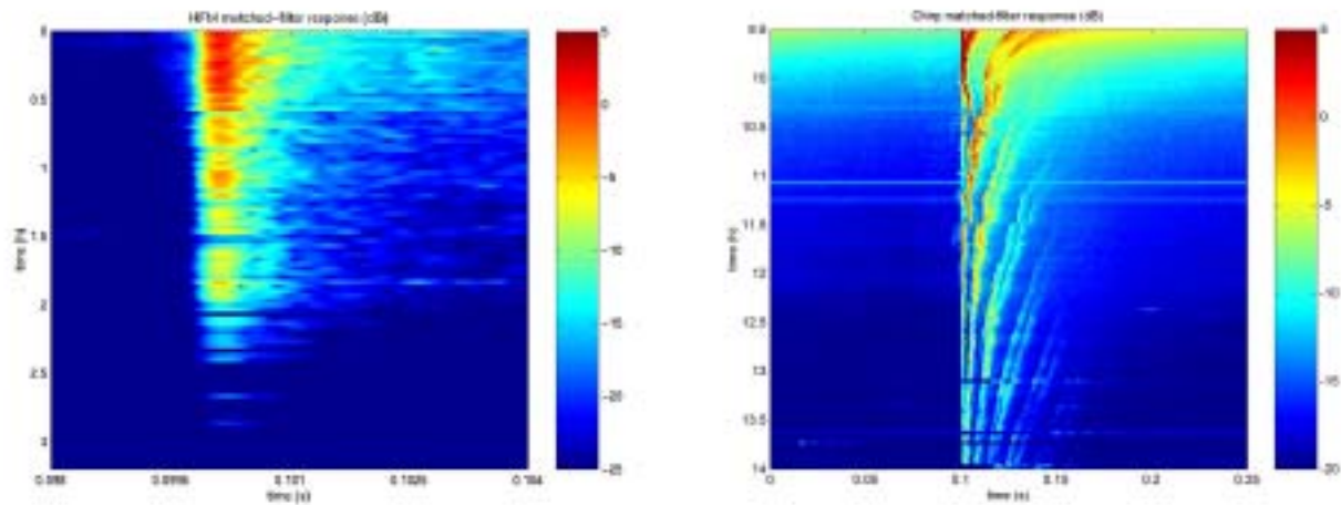
Figure 3: Change in the multipath structure over the course of the day, during which time source/receiver separation increased from about 0-5 km. Ship Island test (left), Coronado Bank test (right).
