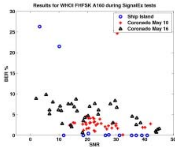
Figure 4: Bit-Error Rate vs. Signal-to-Noise Ratio in 3 separate tests (involving different multipath spread).
