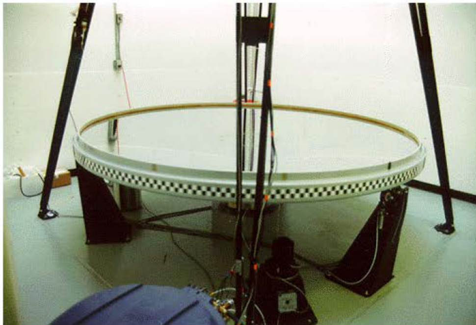
Figure 2: Photograph of the 2.7 meter diameter LMT lidar collector inside the HIPAS lidar building, under a glass sky light for winter -40°C operation.
