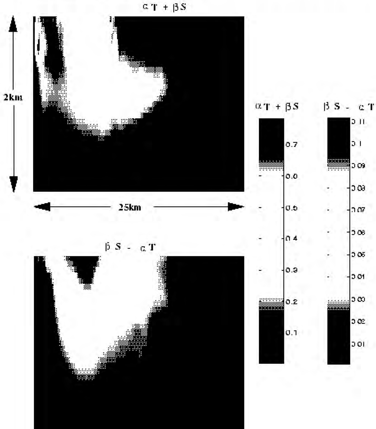
Figure 2. Root mean square values of (a) \alpha T + \beta S and (b) \beta S - \alpha T = (\rho - \rho_0) / \rho_0 .
