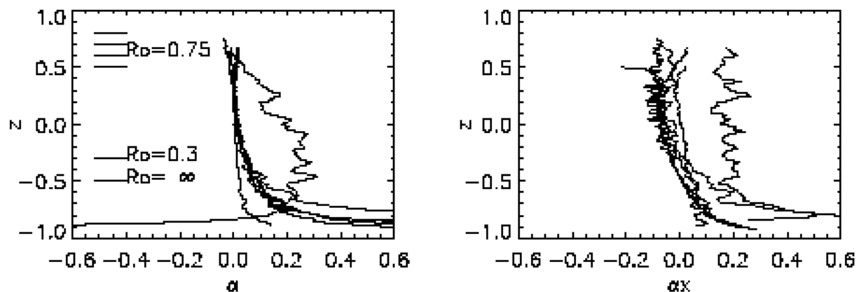
Figure 1. (a) The entrainment coefficient \alpha = \frac{V_e}{W} where V_e is the entrainment velocity, and W is the vertical velocity of a plume, and (b) the mixing coefficient \alpha_x = \frac{U_x}{W} where U_x is the mixing velocity and W is the vertical velocity of a plume.
