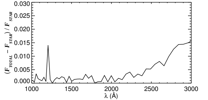
Fig. 2. The model fraction of the disk flux contribution in the 1000 – 3000 Å interval computed by dividing a model containing the disk contribution by the purely photospheric model.
