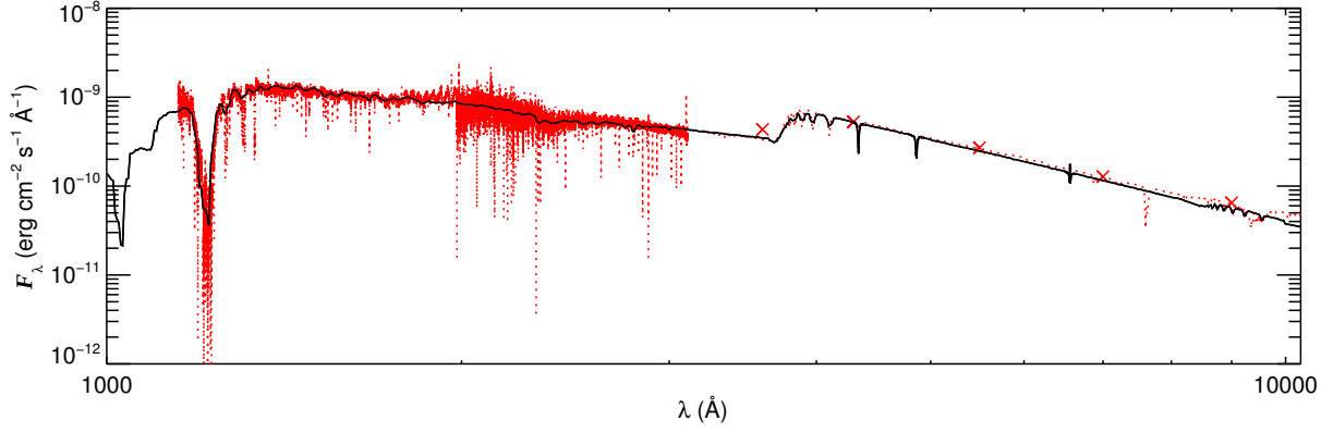
Fig. 3. The parametric ( n = 3.5 ) model fit (solid black) to the average IUE and HPOL data (dotted red). The average HPOL spectrum was scaled to the V-band photometry. The broadband UBVR photometry is plotted with red crosses.
