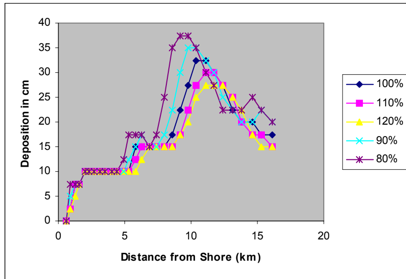
Figure 2. Net deposition during simulated series of storms along a cross-shelf transect. . 100% indicates the wave height used in simulation is from real storm data, while others are simulated runs with increased or decreased wave heights.
