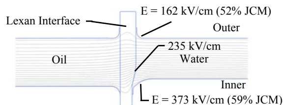
Figure 9. Original stepped pfl inner and diaphragm contours.
