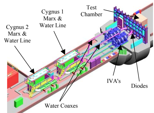
Figure 1. The planned Cygnus underground facility configuration.
