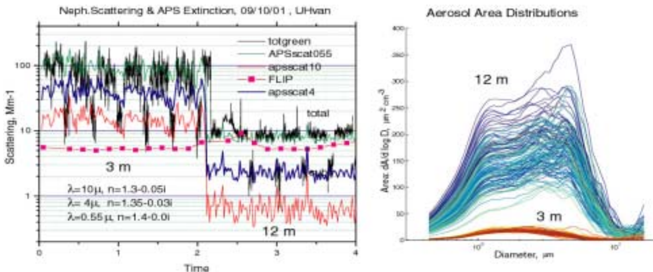
Figure 4. Comparison of sampling switched from 3m vs. 12m for UH Van for wind at about 100deg. a. Modeled extinction in visible (0.55um) and IR (4 and 10um) at 3m and 12m compared to measured (excellent agreement for measured and modeled data, over an order of magnitude greater extinction for 3m aerosol in 10um IR); b. Aerosol area distributions at 3m and 12m
