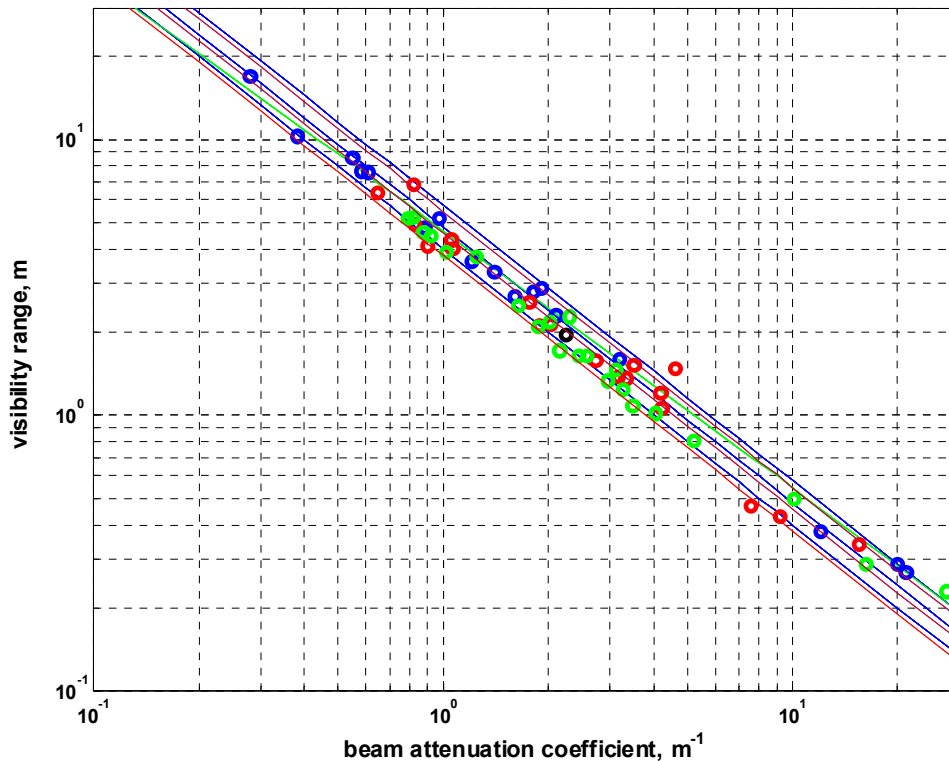
Figure 1.] Graph:Horizontal visibility of a 200 mm diameter black target is shown to have an excellent inverse correlation with photopic beam attenuation as obtained from proxy measurements at 550 and 532 nm. Blue points, Davies-Colley, “green” c-meter; red points, Zaneveld, c(532)*0.9+0.081 ; black point, Twardowski c(532)*0.9+0.081 ; green points, Pegau, c(532)*0.9+0.081 ; blue lines visibility range = y = 4.8/\alpha and +/- 20% lines; green line visibility range = y = (5.207 - 0.368 \ln y)/\alpha ; red lines visibility range = y = 4.55/\alpha and +/- 20% lines; r^2 = 0.985 .]
