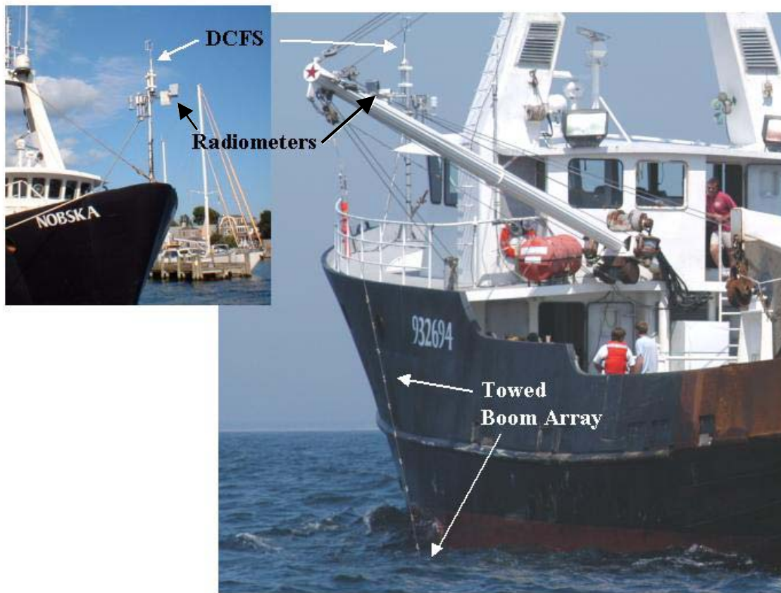
Figure 3. Some of the instrumentation deploy off the Nobska during the IOP. The bow mounted instrumentation included a sonic anemometer, an infrared hygrometers, and infrared radiometers. The boom array towed a string of temperature sensors (T-chain) between the surface and a depth of 20 m. The Nobska crew also deployed 5 surface drifters instrumented with T-chains during the IOP cruises. Results from these instruments are shown in Figs. 7 through 9.
