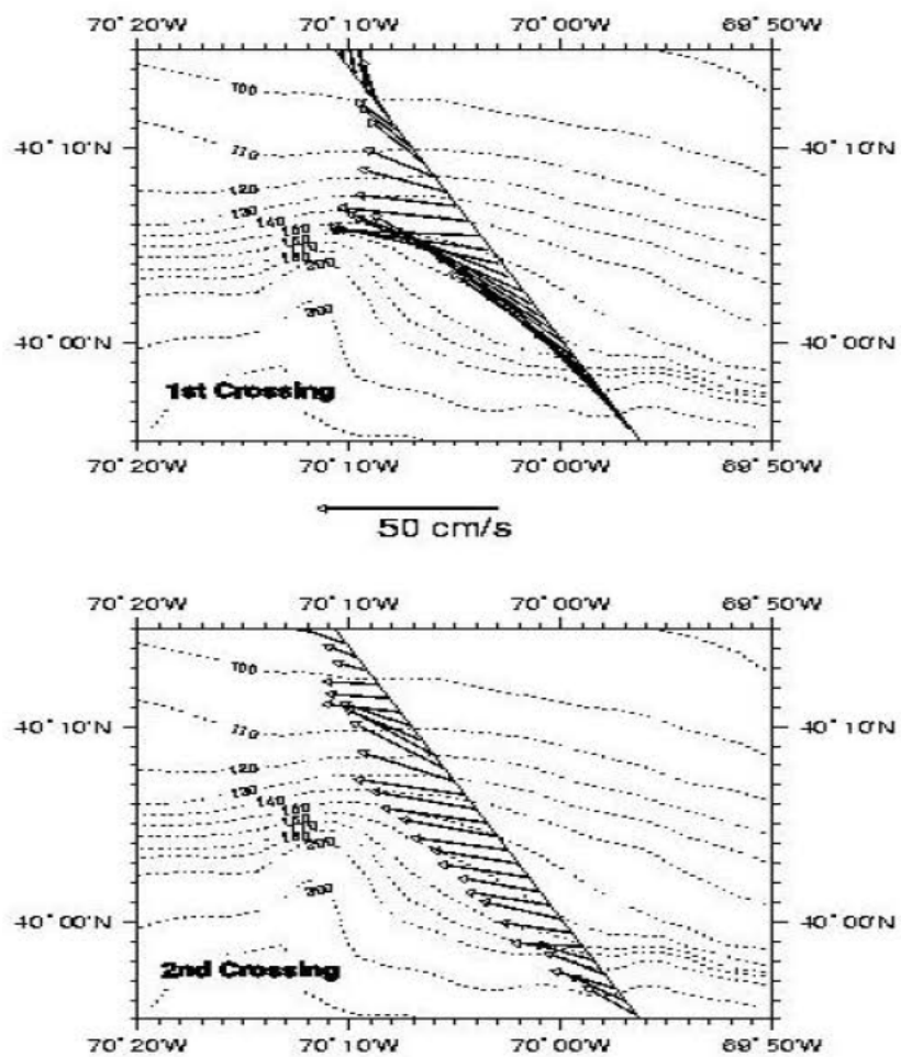
Figure 2: Depth-Integrated velocity of the shelfbreak current during the first PRIMER cruise (from the shipboard ADCP ). The two sections are separated by three days, and sampled two different phases of a meander.
