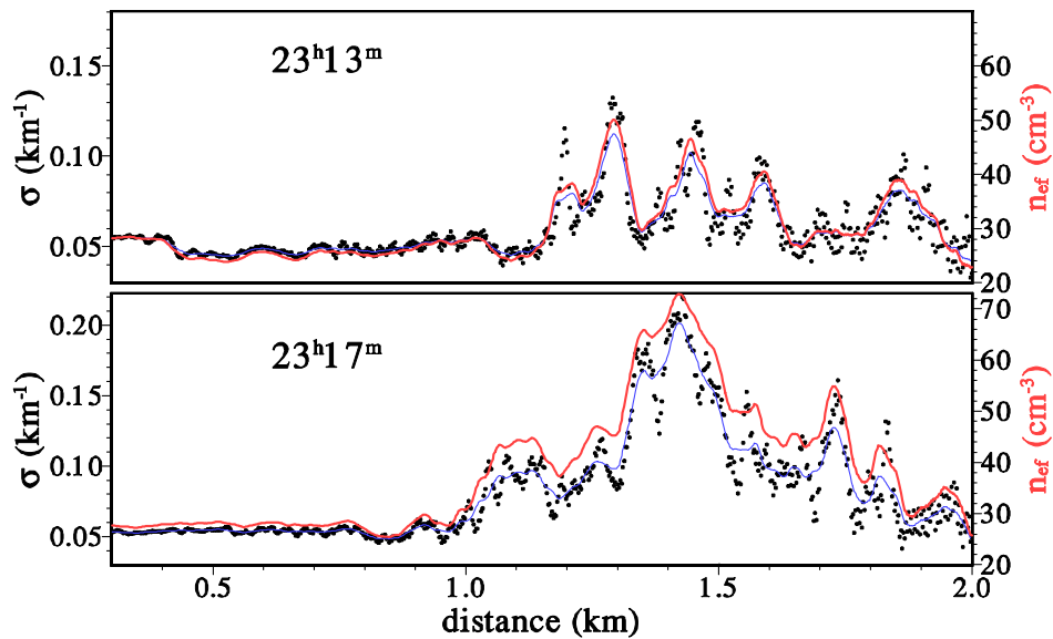
Fig.4. Behavior of n_{ef} along horizontal lidar trajectories.
