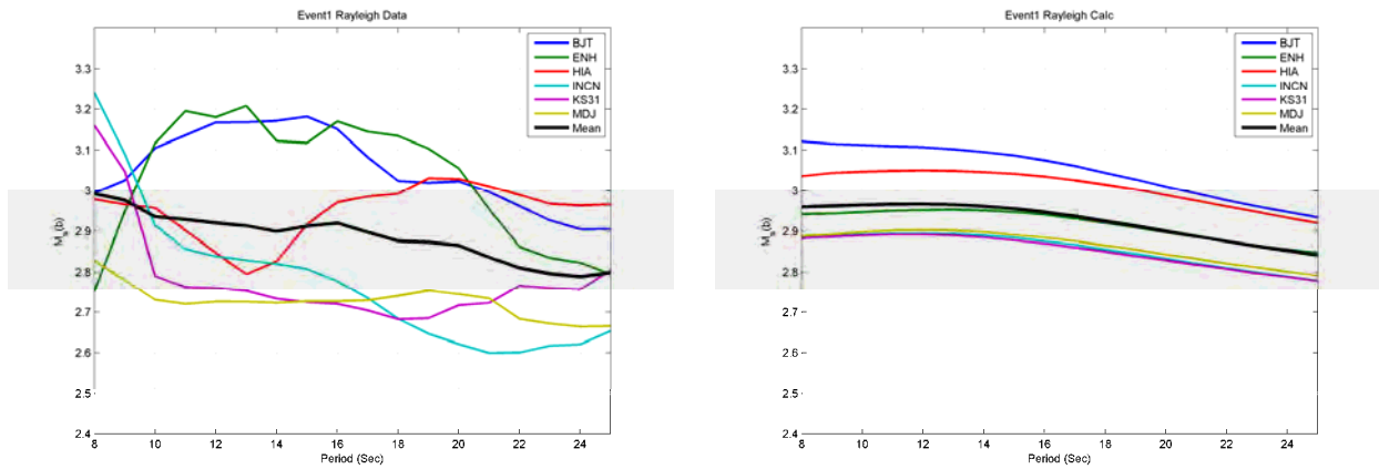
Figure 33. Rayleigh wave data from North Korea event #1 (left), and predicted data from moment tensor inversion (right).
