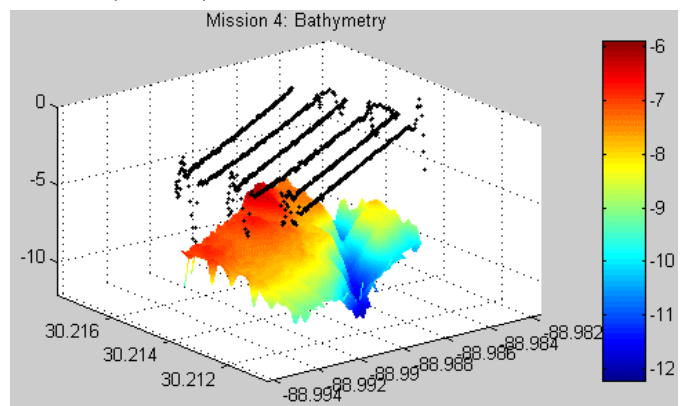
Fig 1 Bathymetry Data from Ship Island reveals an inshore channel 5 meters deeper than the surrounding area
