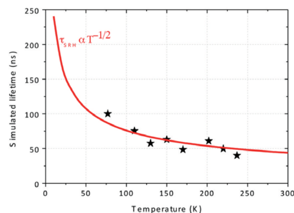
Figure 3 Simulated lifetime as a function of temperature (stars) and the T-1/2 law (solid line)
