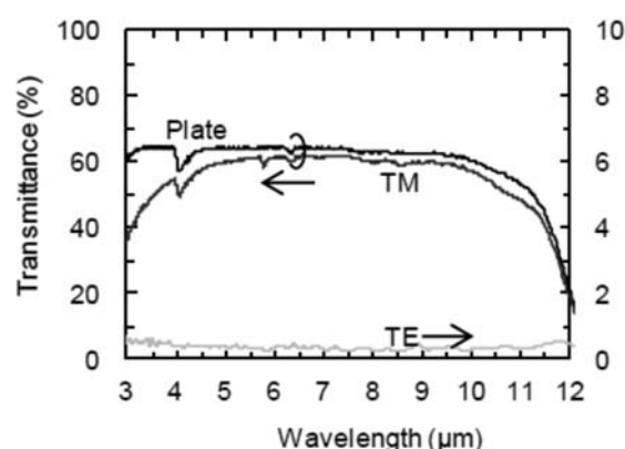
Fig. 3: Transmission spectra of the fabricated element and a chalcogenide glass substrate (2 mm thickness). TE and TM indicate the polarization directions.
