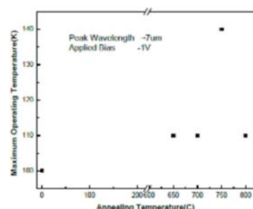
Fig. 4 Maximum operating temperature vs annealing temp of the coupled QDIP
