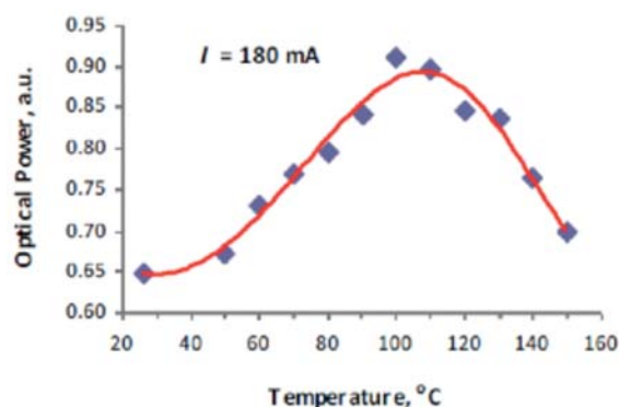
Fig. 2. Experimental temperature dependence of optical power for n-GaSb/Al(As)Sb/InAsSb/Al(As)Sb/p-GaSb QW heterostructure at 180 mA drive current.
