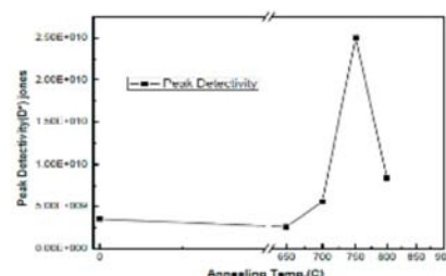
Fig. 5. Peak detectivity of as-grown and annealed QDIP. One order enhancement in D^* is observed 750°C annealed QDIP.
