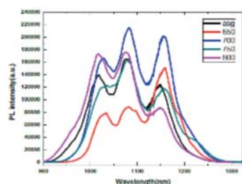
Fig. 2 Low temperature PL shows multimodal distribution of QDs
