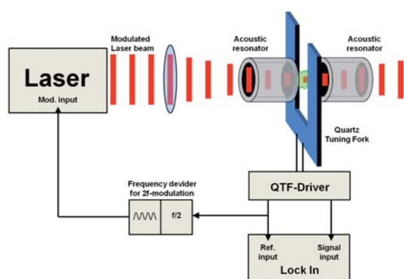
Fig. 1. Scheme of a 2f QEPAS setup with simultaneous electrical co-operation.
