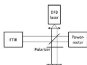
Fig. 1. Experimental set-up for optical feedback. The external cavity can be tuned from 10 to 50 cm.
