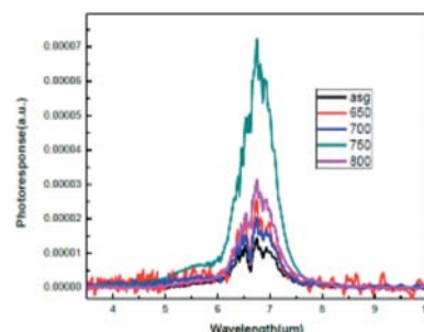
Fig. 3. Spectral response of all the samples measured at 80 K. 750°C annealed QDIP shows 5 times enhancement.
