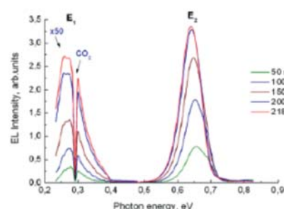
Fig.2. Electroluminescence spectra under forward bias.
