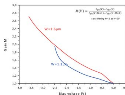
Figure 4. Gain measurement for two different multiplication layer thicknesses.
