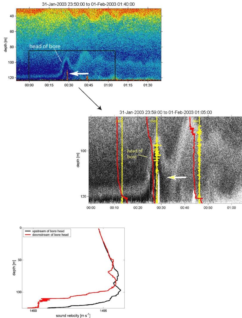
Figure 2 – A highly turbulent and undular bore. Upper plot shows acoustic backscatter image made while maintaining station over a position in 120 m of water depth on the continental shelf. This record is 2 hours long and shows the propagation shoreward of an internal undular bore over the bottom. Beneath this is an expanded plot with CHAMELEON profiles of turbulent shear (yellow) and density (red) through the bore. Sound speed profiles computed across the head of the bore are shown at bottom.
