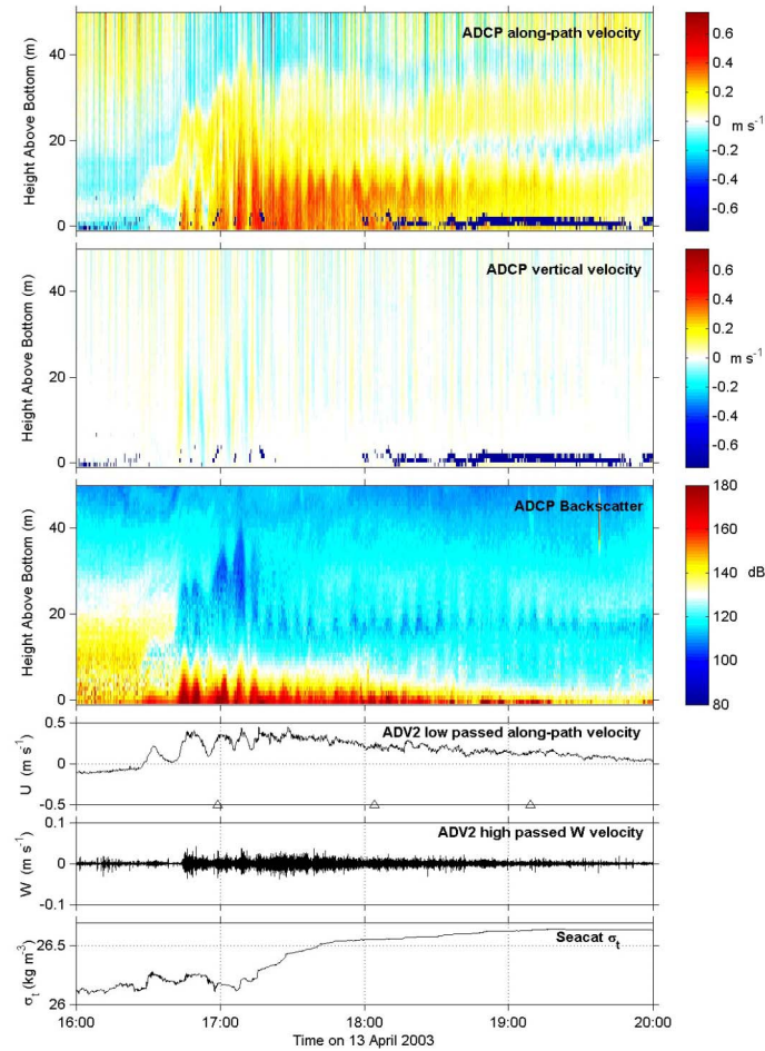
Figure 3 – Time series observations from our bottom lander deployed in 100 m water depth in April 2003. Top panel - shoreward velocity (peak speeds are 0.5 \text{ m s}^{-1} ) as a function of height above bottom; 2 nd panel - vertical velocity; 3 rd - acoustic backscatter; 4 th panel - lowpassed velocity record from an Acoustic Doppler Velocimeter (ADV) 1 m above the bottom; 5 th panel - highpassed record from the ADV showing the variability of the turbulence within the bore; bottom panel - density 1 m above bottom;
