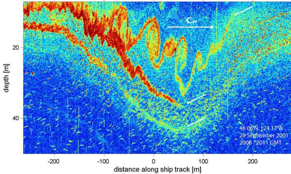
Figure 1 - Example acoustical snapshot of a propagating internal solitary wave within which is embedded a sequence of rollups identical to Kelvin-Helmholtz instabilities observed in the lab and in simulations. Vertical scale of the largest is > 10 m; horizontal scale (in the direction of wave propagation) is \sim 50 m. Toward the wave's trailing edge, rollups are less coherent but contribute greater backscatter signal, suggesting breakdown to turbulence. At greater depth, denoted by arrows, are two more layers of bright backscatter. These are presumably the same phenomenon, but smaller scale. The echosounder resolution does not permit a clear depiction of rollups in these thin interfaces.
