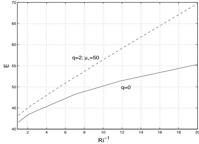
Figure 1: Energy density E vs. Ri^{-1} for q=0 and q=2 and \mu_* = 50 . Environmental parameters are f/N=0.06 , slope angle \gamma=0.1 , N=5.24 \cdot 10^{-5} \text{ s}^{-1} . The overall incident flux is 17.3 \text{ mW m}^{-2} .
