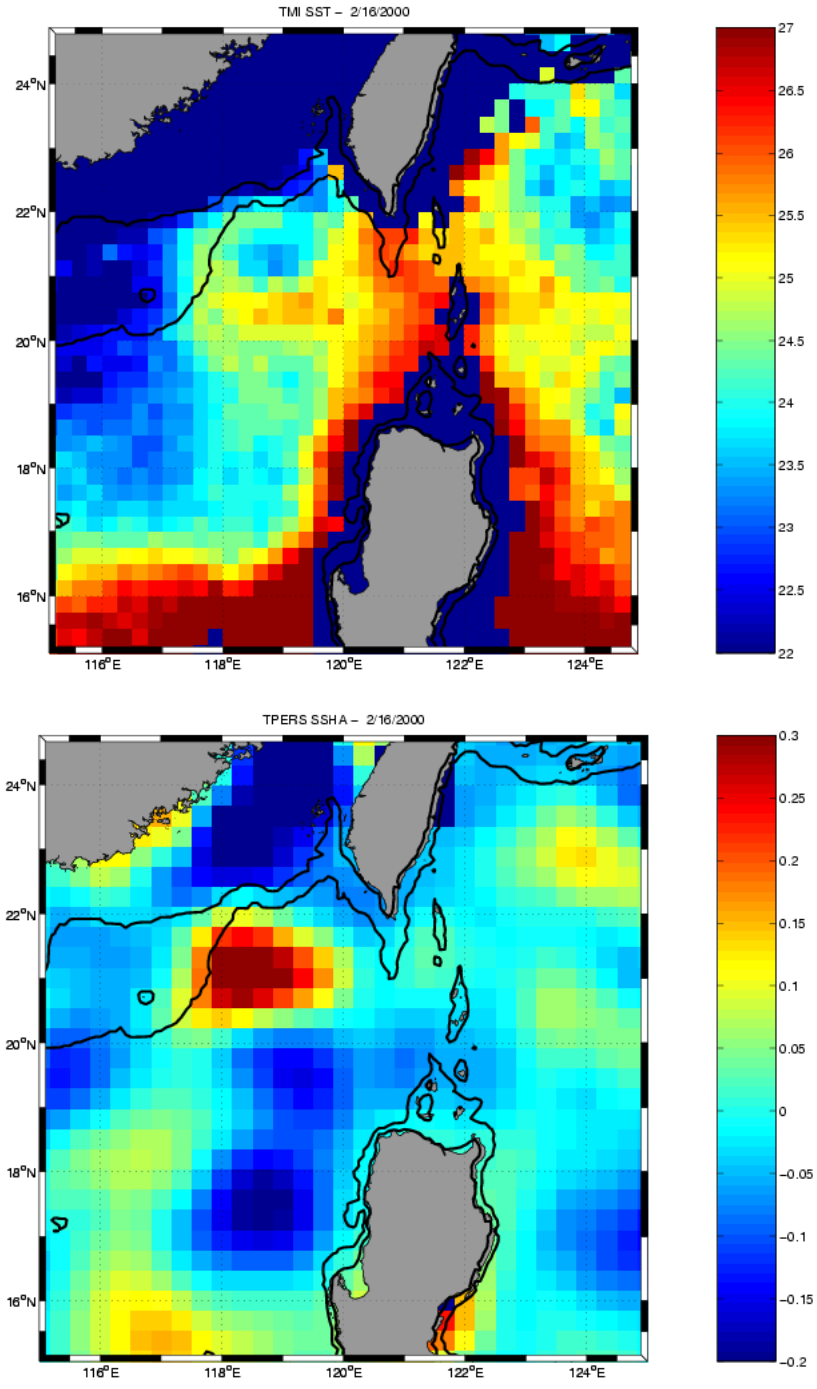
Figure 1. Sea surface temperature (top) and sea surface height anomalies (bottom) showing the large scale anti-cyclonic circulation formed from a Kuroshio intrusion during the winter prior to the 2000 ASIAEX pilot program.
