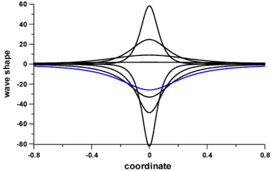
Figure 1b Solitary wave shape for positive cubic nonlinearity.
