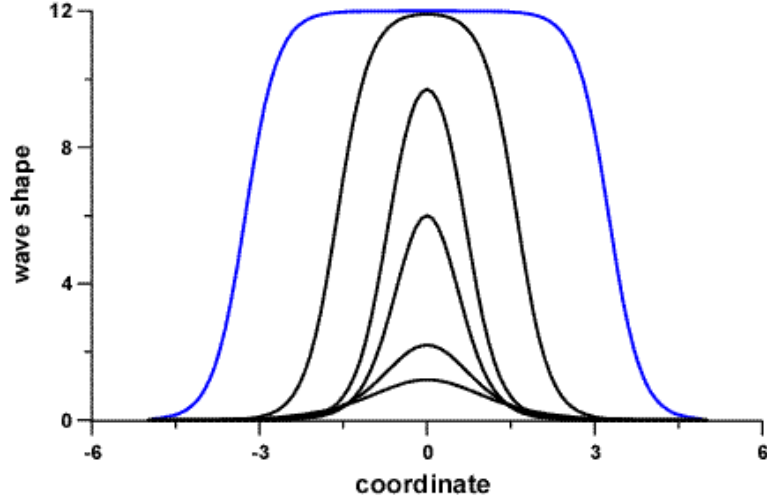
Figure 1a Solitary wave shape for negative cubic nonlinearity.
