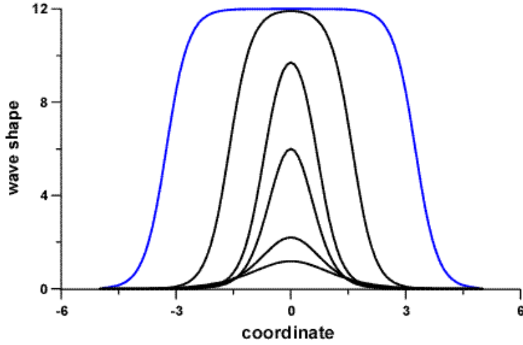
Figure 1a Solitary wave shape for negative cubic nonlinearity.
