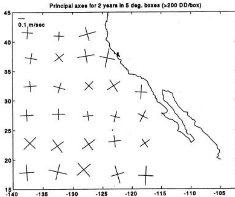
Figure 3. Current principal axes computed on a 5^\circ by 5^\circ grid over the same 2-year period.
