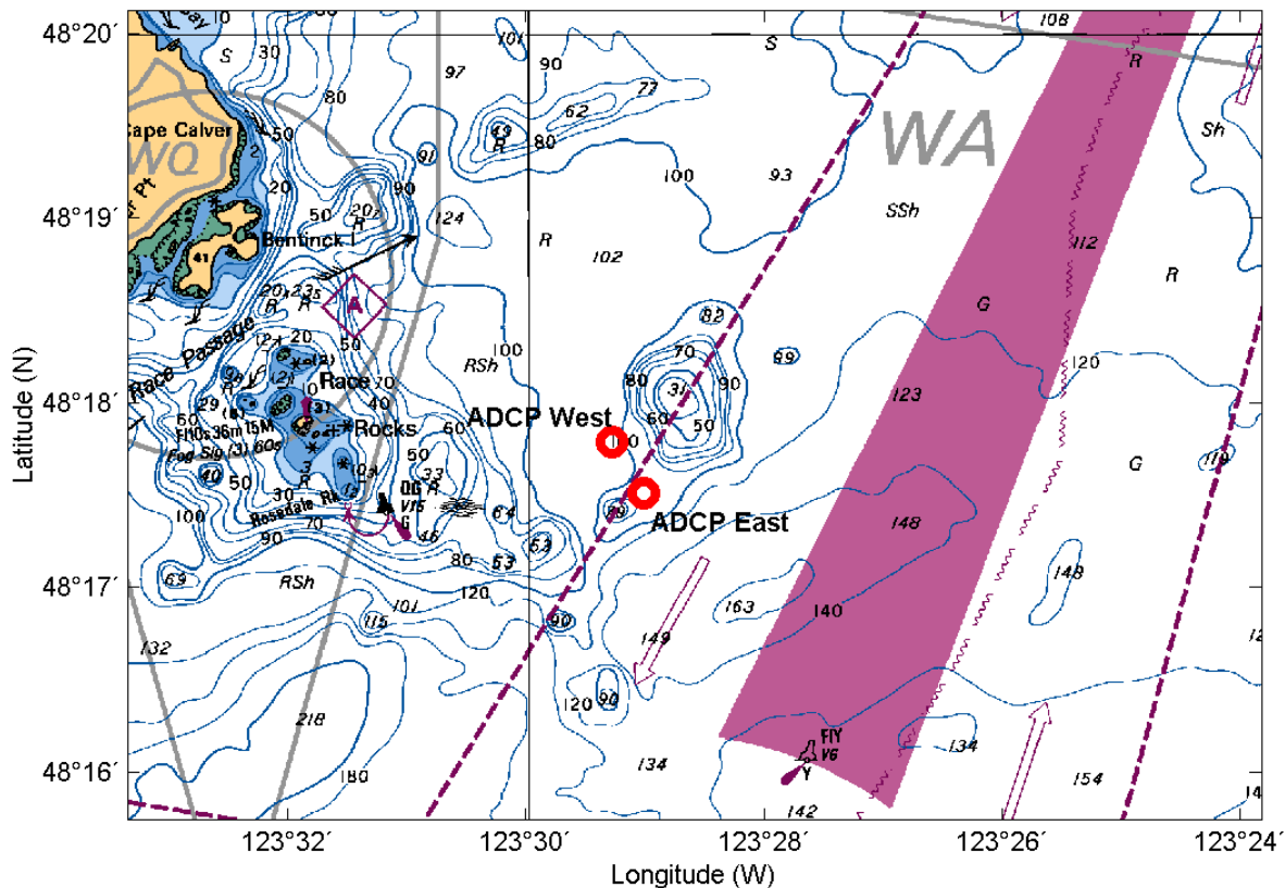
Figure 1. An isolated bump in the strong stratified tidal flows in Juan de Fuca Strait. The location of moored ADCPs is shown.
