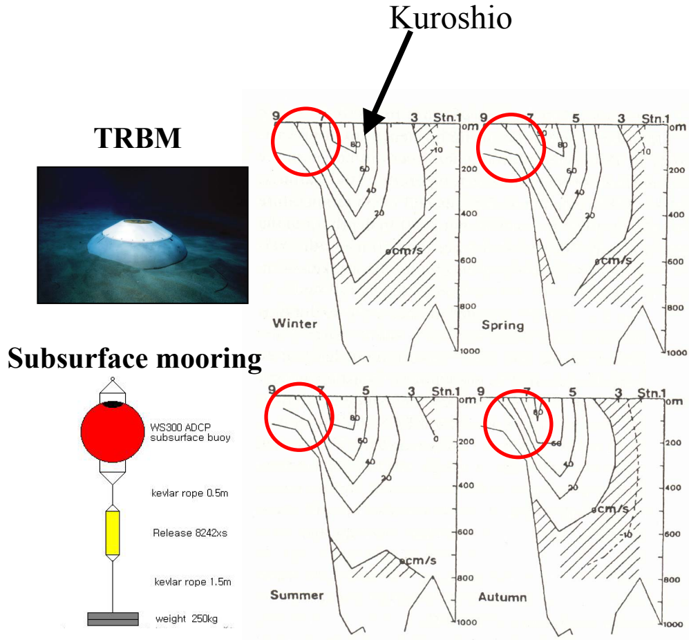
Figure 1. Vertical sections (right) of seasonal mean geostrophic current normal to the PN-line referred to GEK velocity (from Ichikawa and Beardsley, 2002). Red circles denote areas influenced by the northeastward flowing Kuroshio over the outer continental shelf. Acoustic Doppler current profilers housed in trawl-resistant bottom mount (TRBM; upper left) and subsurface buoy (lower left) will be used to measure this part of the Kuroshio. Shaded area indicates southwestward current.
