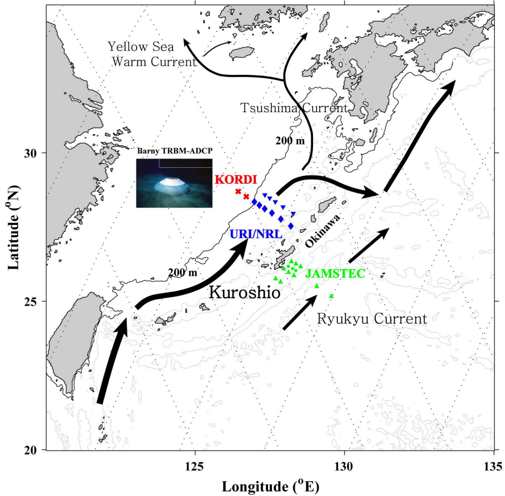
Figure 2. Schematic paths of the Kuroshio and its branches in the ECS together with locations of KORDI's ADCP moorings (red crosses) in the ECS and the IES array (blue diamonds and triangles) near the PN-line.
