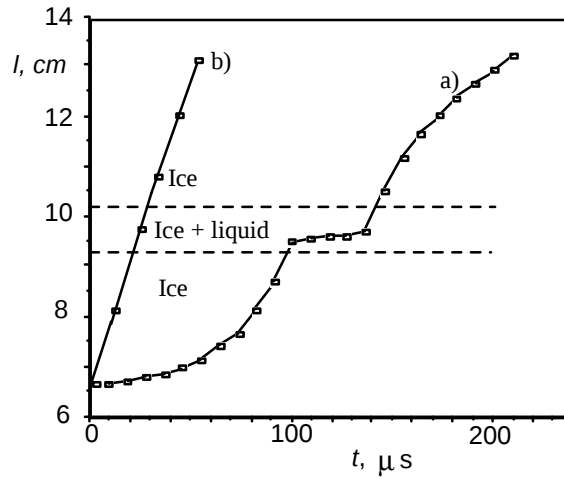
Figure 4. a) Crack length vs time in a sample of freshwater ice with a hole filled with liquid fluorocarbon. T = -10\text{ C} . b) Same with an empty hole.
