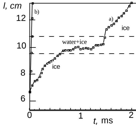
Figure 4. a) Crack length vs time in a sample of freshwater ice with a hole filled with liquid fluorocarbon. T = -10\text{ C} . b) Same with an empty hole.
