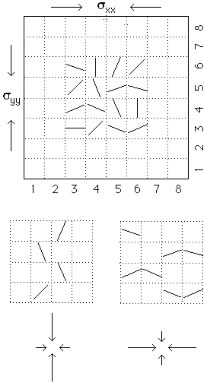
Figure 3. Schematic of random oriented flaws together with "activated" flaws for differently oriented maximum principal stresses.
