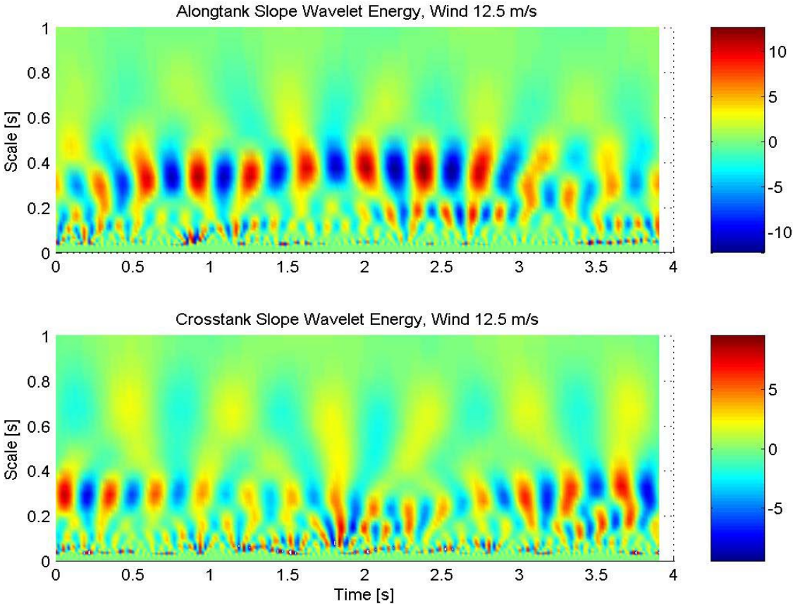
Figure 1. Morlet wavelet spectrum of wind generated waves, Wind velocity 12.5 m/s. Top plot alongtank energy, bottom plot cross-tank energy. Scale is proportional to wave period. Dominant wind waves are centered at 0.3 s. Bragg waves are at scales less than 0.1 s. Positive energies denote increasing slopes, Negative energies denote decreasing slopes.
