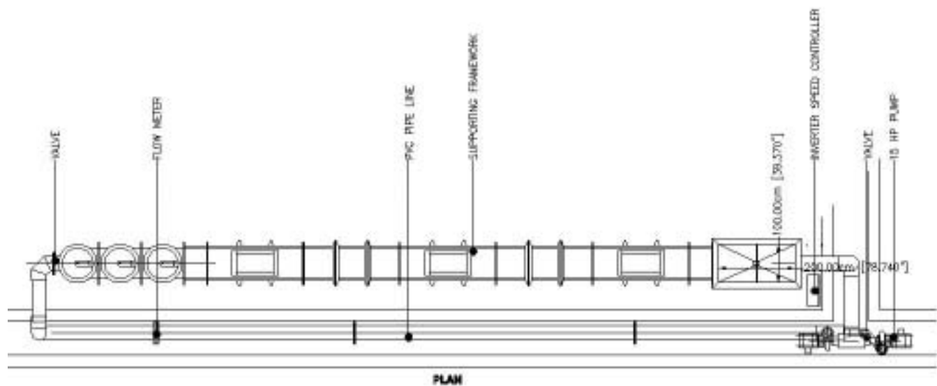
Figure 2. Large Oscillating Water-Sediment Tunnel, LOWST (top view)
