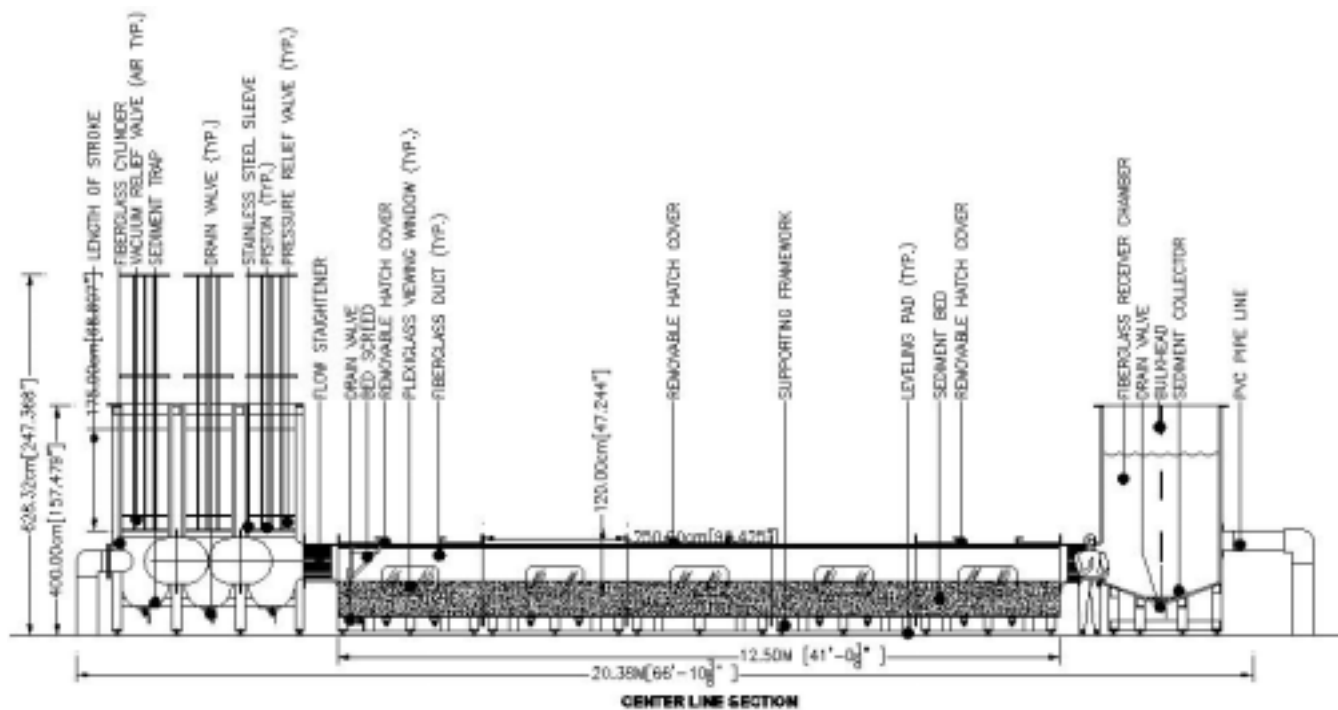
Figure 1. Large Oscillating Water-Sediment Tunnel, LOWST (side view)
