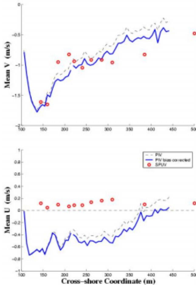
Figure 2. Comparisons spanning the width of the surf zone between 30-minute mean surface velocities estimated from raw (dashed lines) and bias-corrected (blue lines) PIV methods and time series obtained from the same location but near the seabed with in situ current meters (red circles). Mean alongshore flow is shown in the upper panel and mean cross-shore flow is shown in the lower panel.
