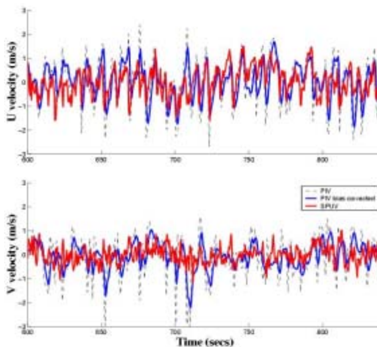
Figure 1. Comparison between 4-minute time series of mean-corrected surface velocities estimated from raw (dashed lines) and bias-corrected (blue lines) PIV methods and time series obtained from the same location but near the seabed with in situ current meters (red lines). Cross-shore velocities are shown in the upper panel and alongshore velocities are shown in the lower panel.
