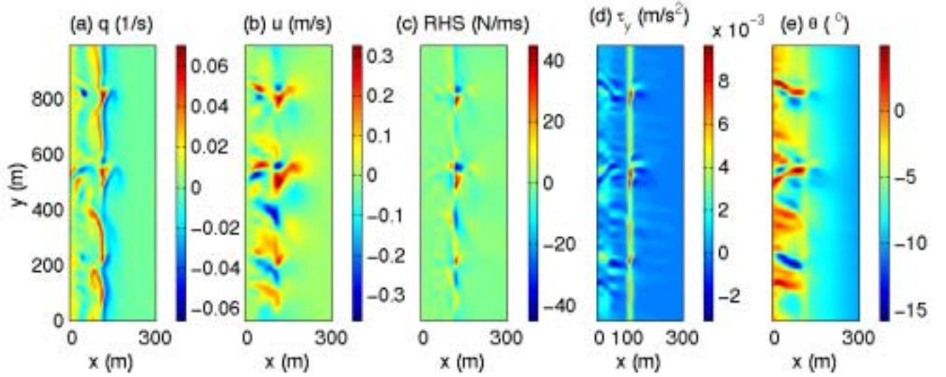
Figure 1: Snapshots for a circulation field involving the instability of a longshore current that flows in the +y-direction. Depicted are (a) the vorticity, (b) the cross-shore velocity, (c) the wave-current interaction terms within the energy equation for the wave motion (see Özkan-Haller and Li, 2002), (d) longshore component of the wave forcing, and (e) local angle of wave incidence, where x points offshore and y points alongshore. Of note are areas where the current field performs work on the wave field, causing it to gain energy (red areas in panel (c)). Note that these coincide with offshore directed flow features (panel (b)). These also cause refraction of the incident wave field (panel (e)), which, in turn, cause variations in the wave forcing of the circulation (panel (d)), ultimately leading to strong fluctuations in the velocities near the shoreline, which are absent when wave-current interaction is neglected.
