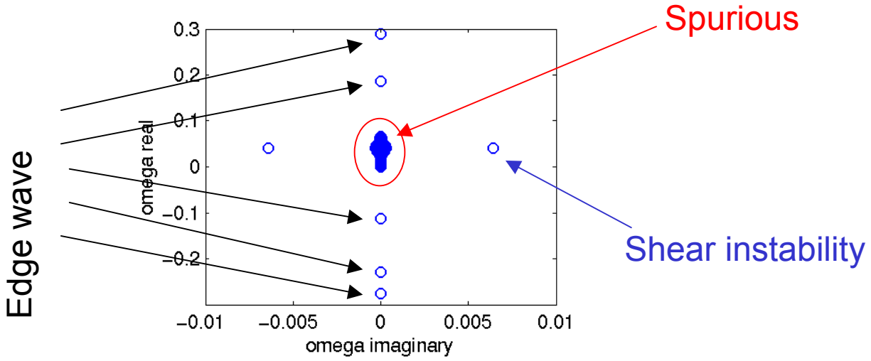
Figure 2: Real part of the radial frequency versus the imaginary part of the radial frequency for motions at radial wavenumber k=0.06 rad/m. Positive imaginary frequencies indicate an exponentially growing mode, negative imaginary frequencies indicate exponentially decaying modes. The edge wave modes, shear instability modes, and spurious modes are marked.
