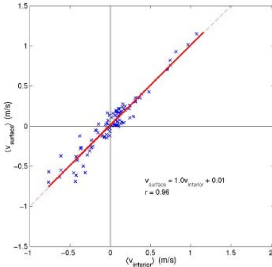
Figure 2. Test of the optical current meter, comparing optical estimates of mean longshore current ( V_{surface} ) to ground truth measurement ( V_{interior} ) from the SandyDuck field experiment (ground truth provided courtesy of R.T. Guza and S. Elgar). The optical technique is unbiased, with an rms error of 10 cm/sec (some of which is true, wind-generated shear). [Data cluster along the 1:1 line, spanning a range from -1 to about +1 m/sec]
