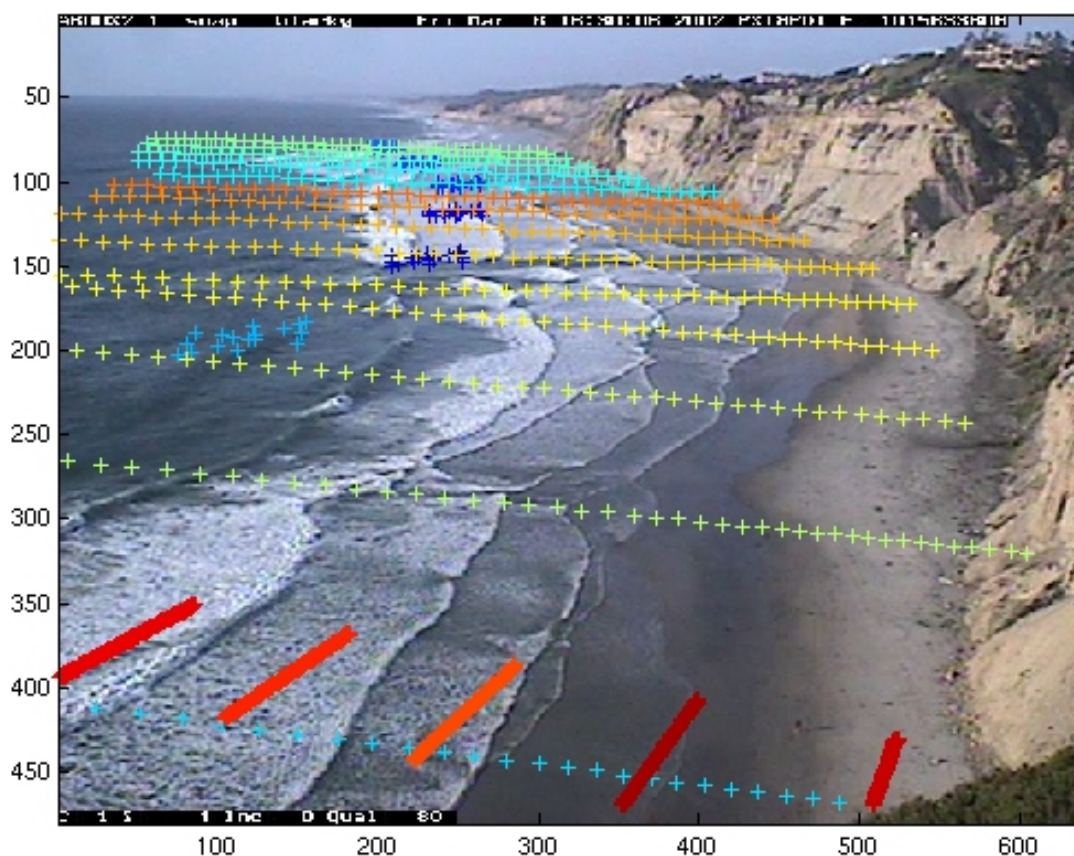
Figure 1. Initial pixel instrument array at Black's Beach, CA. Cross-shore lines allow bathymetry estimation, alongshore (red) lines provide estimates of the longshore current, offshore pixel "blobs" measure wave angle of incidence. [View of Black's Beach with superimposed symbols indicating array of pixels to be sampled].
