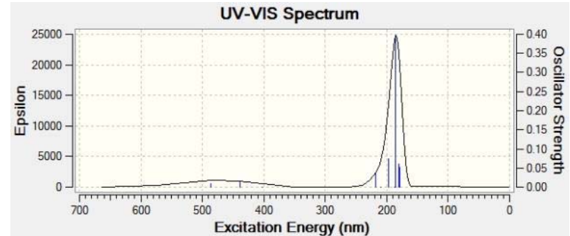
CuCl Calculated Electronic Absorption Spectrum
