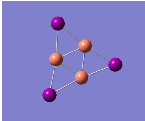
(CuI) 3 – 278.6 cm -1 vibration
