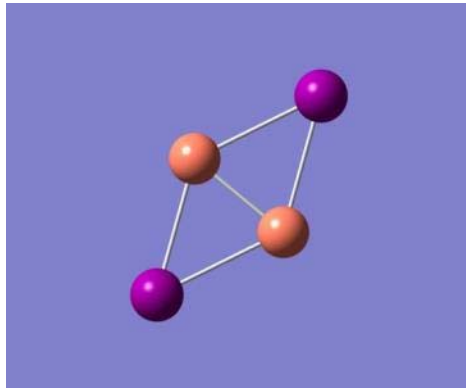
Copper Iodide Dimer (CuI) 2
