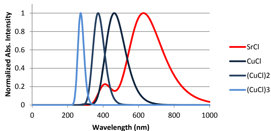
Calculated (CuCl) n Absorption Spectra
