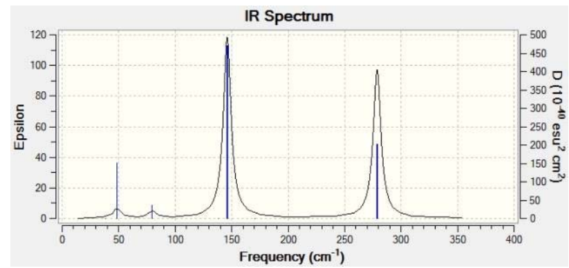
(CuI) 3 Calculated Vibrational Spectrum
