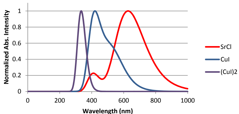
Calculated (CuI) n Absorption Spectra
