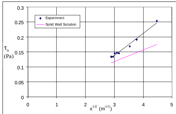
Figure 3. Shear Stress Beneath Surface Film, \tau_o as Measured by the LDV.
