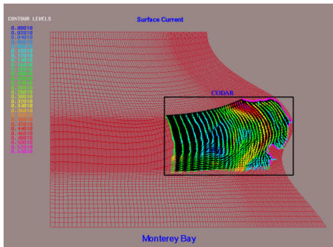
Fig. 2. MOB model-generated CODAR data.
