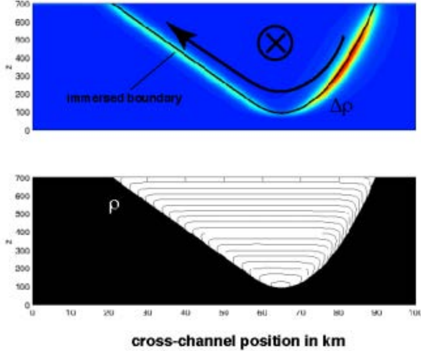
Figure 2. Upper panel (a) shows the density perturbation from a linear profile, emphasizing the heat source just below the immersed boundary. Lower panel (b) shows the total density field that satisfies the required adiabatic condition. The vertical coordinate is in meters.
