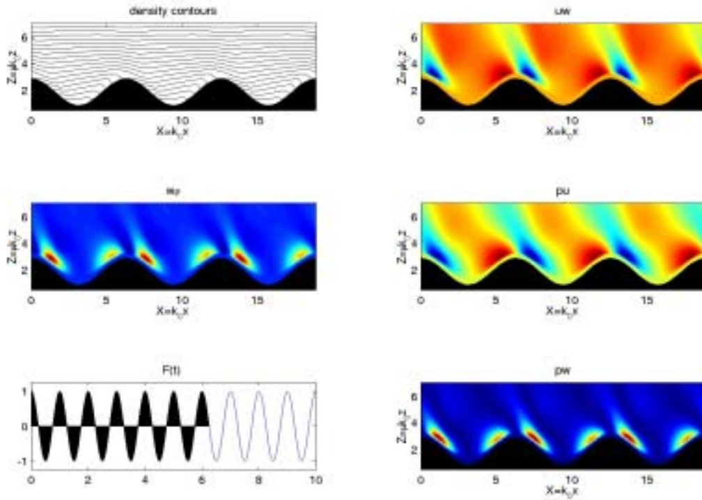
Figure 1: Instantaneous view of generation of internal tide at horizontal scale 2\pi/k_0=2500m at critical slope. The bottom left panel shows the phase of the forcing at the time of the snapshot.
