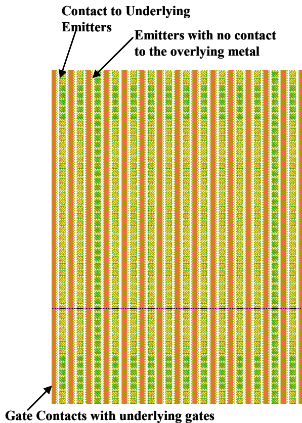
Figure 5. Si SGTO modified emitter cell design [4]
