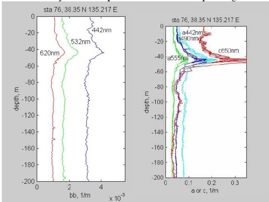
Figure 1. Profiles of spectral inherent optical properties in the central region of the JES. a. Backscatter coefficient obtained with HoboLabs HydrosCat 6. b. Absorption and attenuation coefficient obtained with Wet Labs AC-9.
