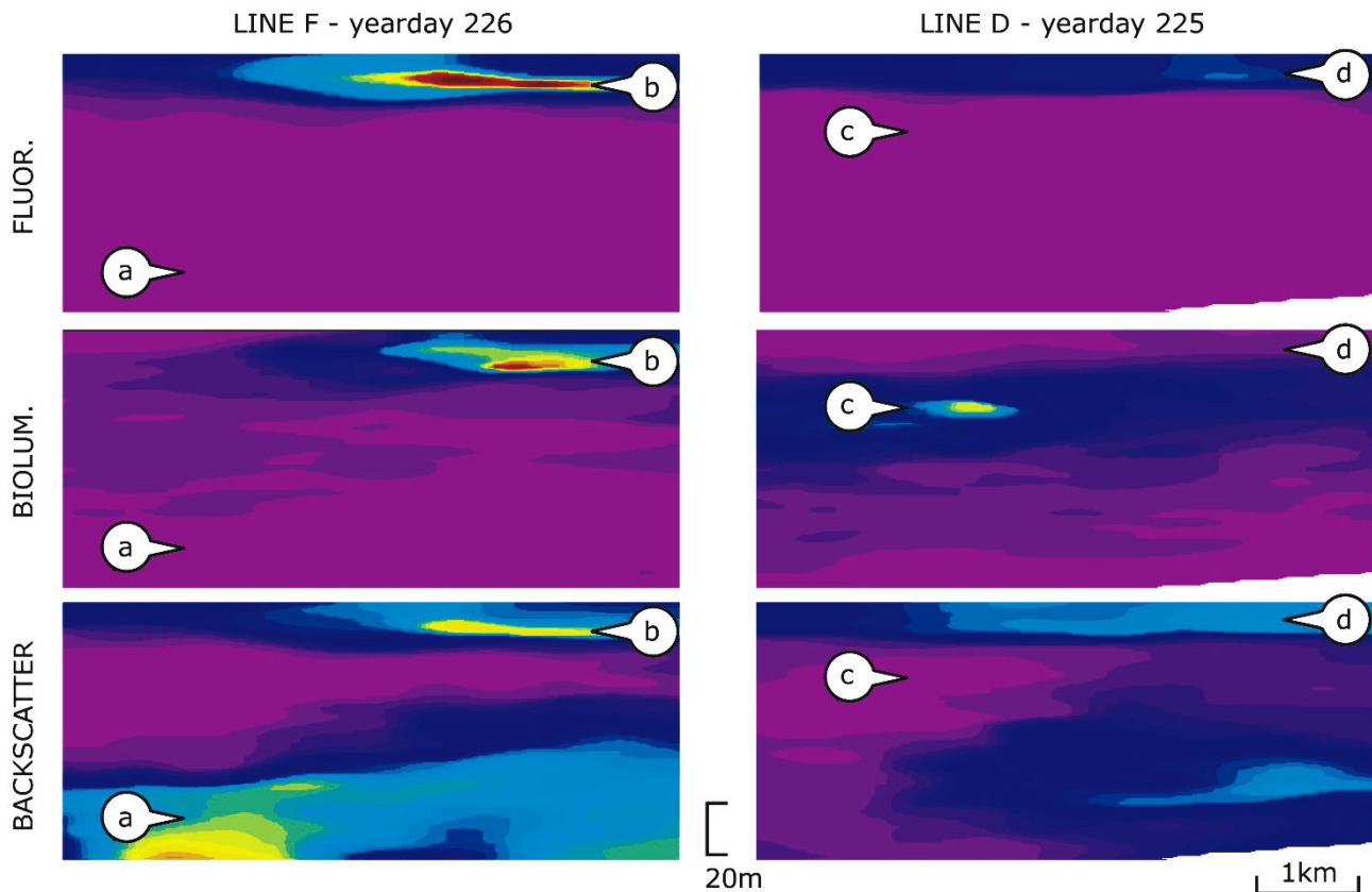
Figure 2. Correlation between features in 2003 AUV Survey Data. In our data, it has not possible to generalize about the spatial relationship between chlorophyll fluorescence, bioluminescence, and optical backscatter across the entire survey domain. (a) Optical backscatter indicates the presence of sediment, lacking fluorescence or bioluminescence, but at times high values (b) of all three measurements may co-occur. We believe these instances indicate dinoflagellate bioluminescence. (c) High bioluminescence may also occur in areas with no detectable particles, either fluorescent or not, and in certain water masses, (d) high fluorescence and backscatter occur in a layer above the region of high bioluminescence.
