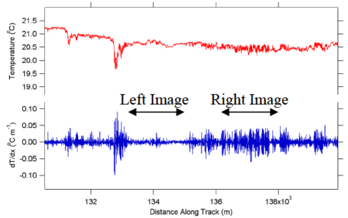
Figure 3. (a) Examples of fine-scale IR imagery as observed from the aircraft under very low wind speed. Each image is roughly 160\text{ m} \times 200\text{ m} and the top of the images is West. (b) Temperature and its derivative measured along the flight track that correspond to the observations in (a).
