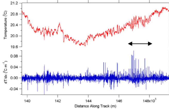
Figure 2. (a) Mosaic of IR images from Snapshot mode showing the successive fronts of ocean skin temperature in the presence of ubiquitous surface slicks observed on 8-22-02 during a period when the wind was 5 \text{ m s}^{-1} from the SW. The top of the mosaic is NE. (b) Point mode temperature and its derivative measured along the flight track that correspond to the observations in (a). The black arrow denotes the region of the coherent ramp structures observed in (a).
