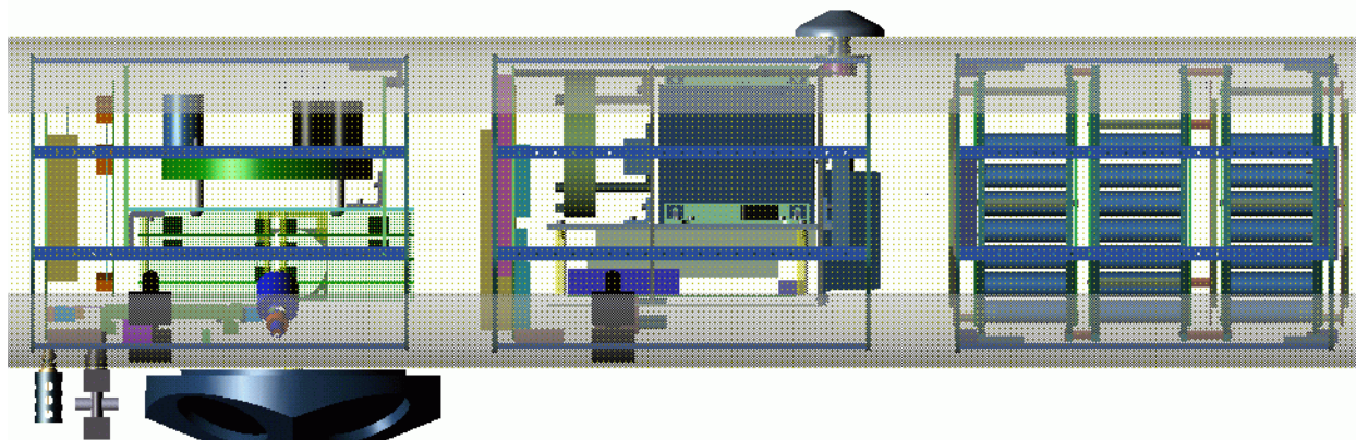
Figure 4.1 In order from left to right: Main computer section including DVL, CTD, and Health Board; Navigation Module including FOG gyros, acoustic modem; Battery section showing NiMH batteries..
