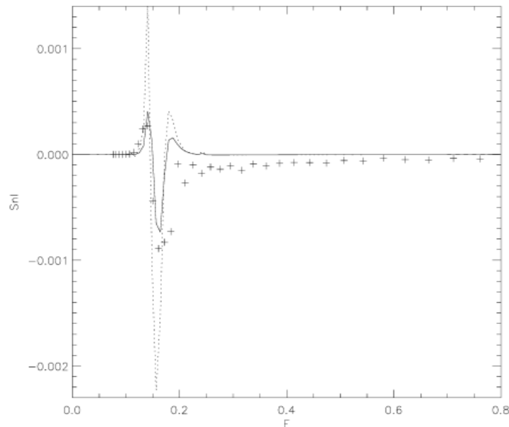
Figure 3. Nonlinear interaction term dependence on frequency at the angle \varphi = 0 . Crosses represent Resio-Tracy results, dashed line -- first generation model, solid line - second generation model.
