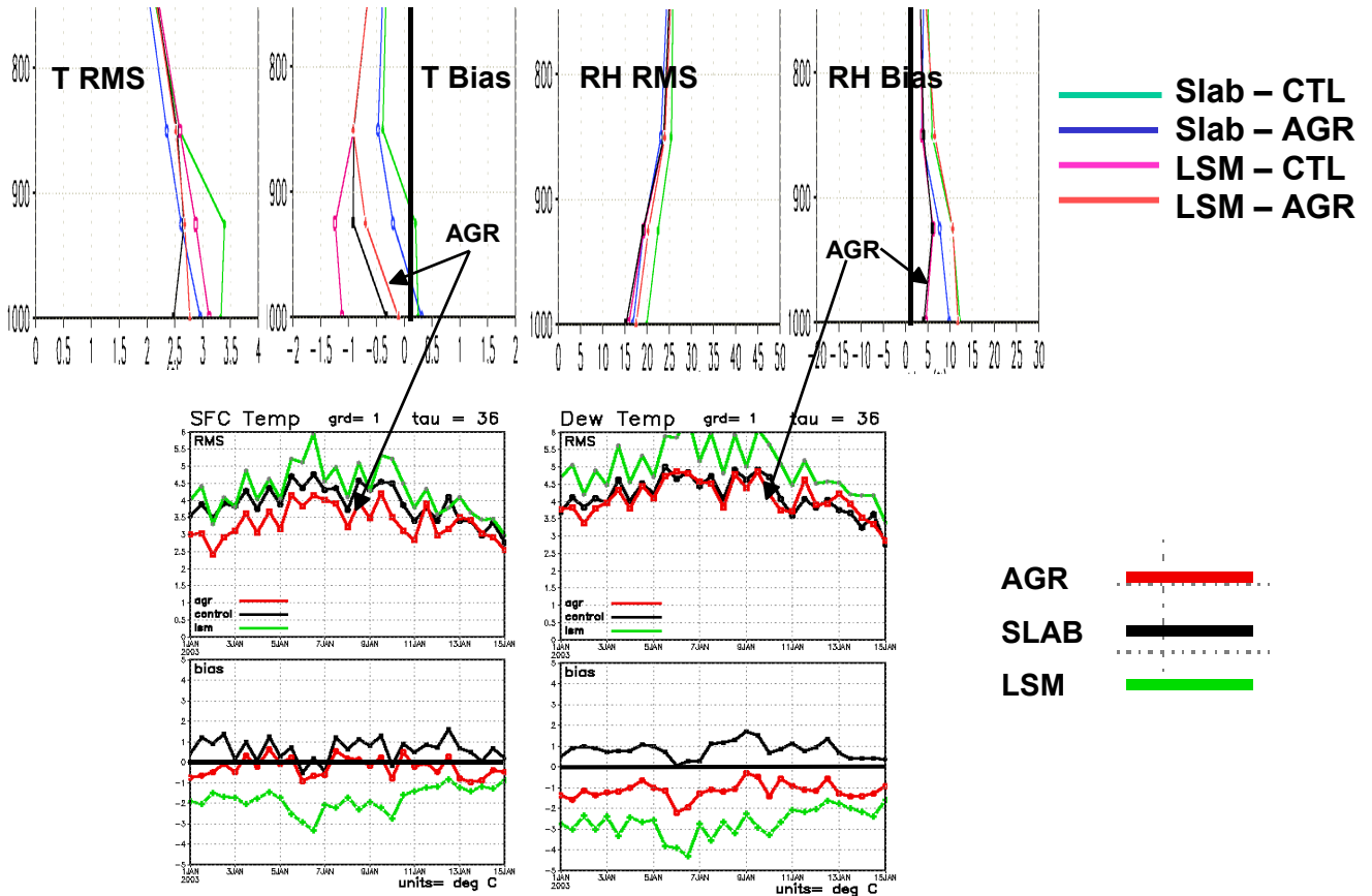
Figure 1. COAMPS lower atmosphere temperature and moisture root-mean-square and bias errors (top four panels). The surface temperature and dew point depression statistics for January 2003 over Europe area are shown in the bottom two panels.
