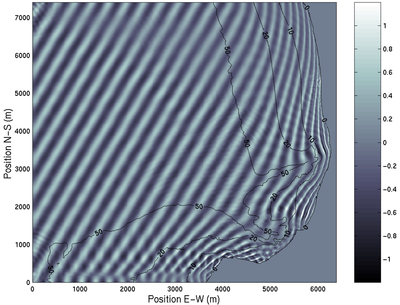
Figure 1 Surface elevation field for a 6 x 7 km region around the NCEX site in La Jolla, CA Monochromatic waves with a period of 17 sec and a significant wave height of 1 m from 295°T are generated at the offshore boundaries. Bathymetry contours show the near-shore canyons.
