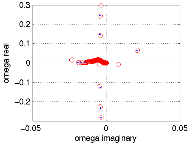
Figure 2: Real part of the radial frequency versus the imaginary part of the radial frequency for motions at radial wavenumber k=0.06 rad/m. Positive imaginary frequencies indicate an exponentially growing mode; negative imaginary frequencies indicate exponentially decaying modes. Edge waves display negative growth rates (due to frictional decay), the shear instability mode displays positive growth rate. Close to the origin there are several instability modes that represent morphological instabilities.
