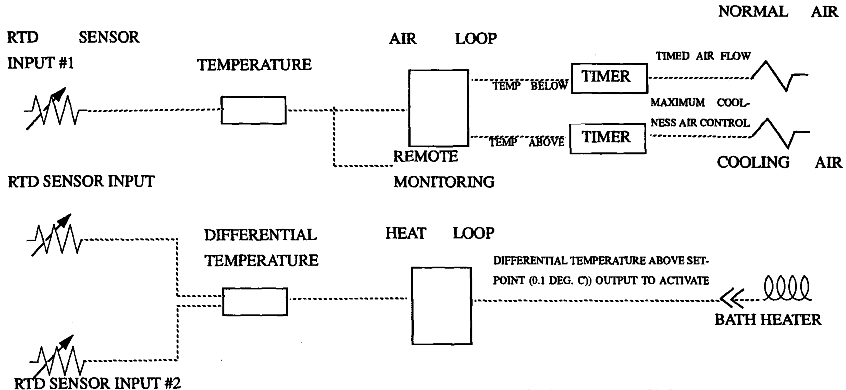
Figure 9 - 2 Functional Control Diagram of Adiabatic Composter Unit Used by Woods End Research Laboratory to Test Compost Mixtures for Contaminated Soil Composting
