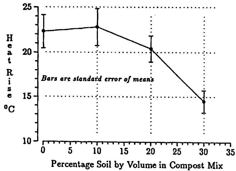
Figure 9 - 4 Relationship of Soil Inclusion Rate in UMDA Compost and Average Temperature Above Ambient Attained Over 30 Days
