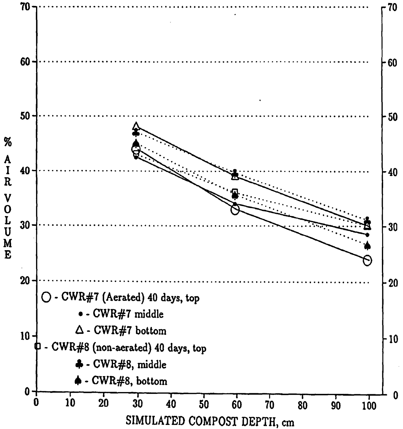
Figure 11 - 3 Compost Air Volume as a Function of Pile Management, Depth in Pile, at Simulated Depths
