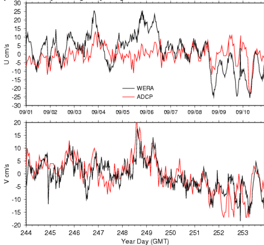
Figure 2. Comparison of surface velocities from WERA with those from 3m bin depth ADCP velocity, 1 to 11 SEP 03. The comparison is favorable except for the roughly 10 cm/s offset in the east-west current component during the passage of Tropical Storm Henri.
