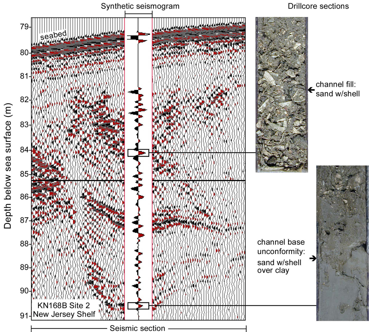
Figure 1. Example seismic reflectors within paleochannel fills on the New Jersey continental shelf. Shown is the chirp seismic section for drillcore Site 2 (wiggles plot), a synthetic seismogram constructed from downcore seismic velocity and density profiles, and photos of two core intervals at seismic discontinuities. The upper interval corresponds to a depositional reflector, sand and shell emplaced when the channel was being backfilled. The lower interval shows an erosional reflector, stiff clay that was eroded when the channel incised the shelf.
