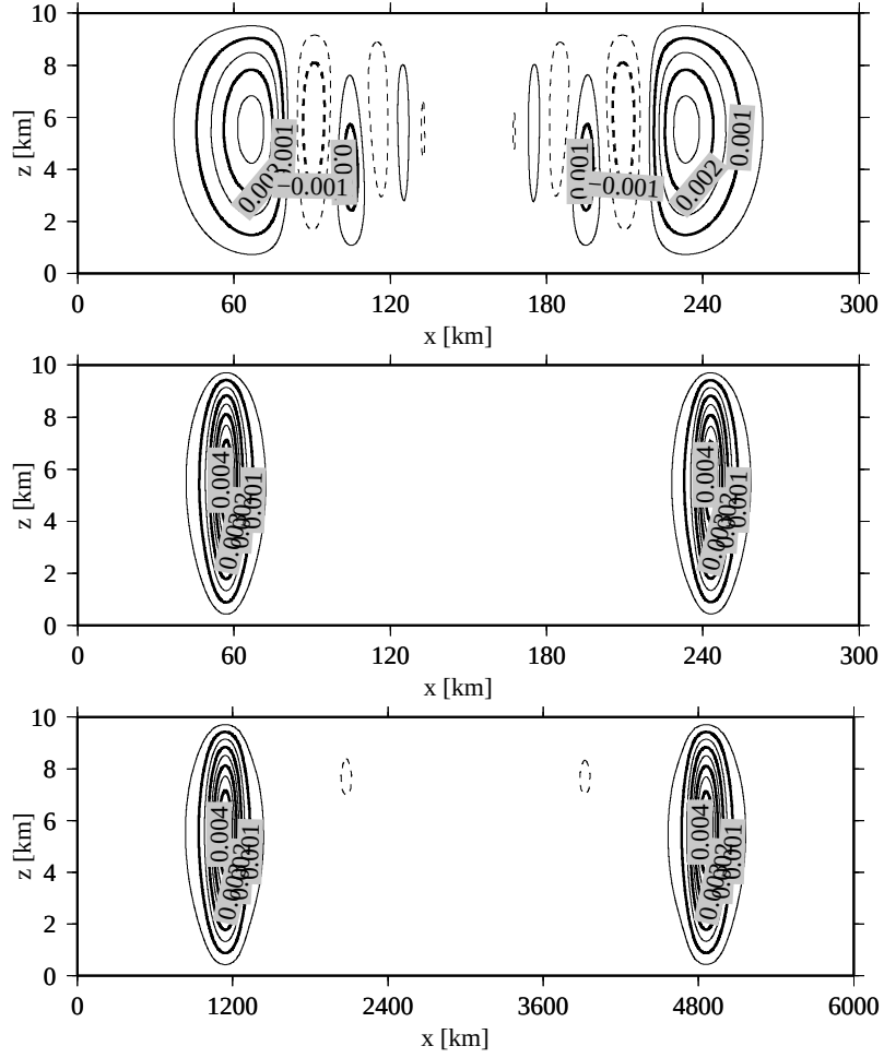
Figure 2: Gravity waves, section 4.1, model results for potential temperature perturbation \theta , contour interval 5 \times 10^{-4} \text{K} , top: short channel, T = 3000 \text{s} , non-hydrostatic system, middle: short channel, T = 3000 \text{s} , hydrostatic system, bottom: long channel, T = 60000 \text{s} , non-hydrostatic system; In the long channel, the non-hydrostatic and hydrostatic plots look the same. Thus, the hydrostatic plot is omitted.
