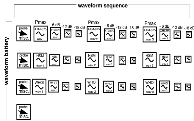
Figure 2. The waveform battery is a concatenation of many communication waveforms and compound probes. Source-level reduction producing diminishing SNR at the receiver and reveals failure modes in the demodulation and decoding process.
