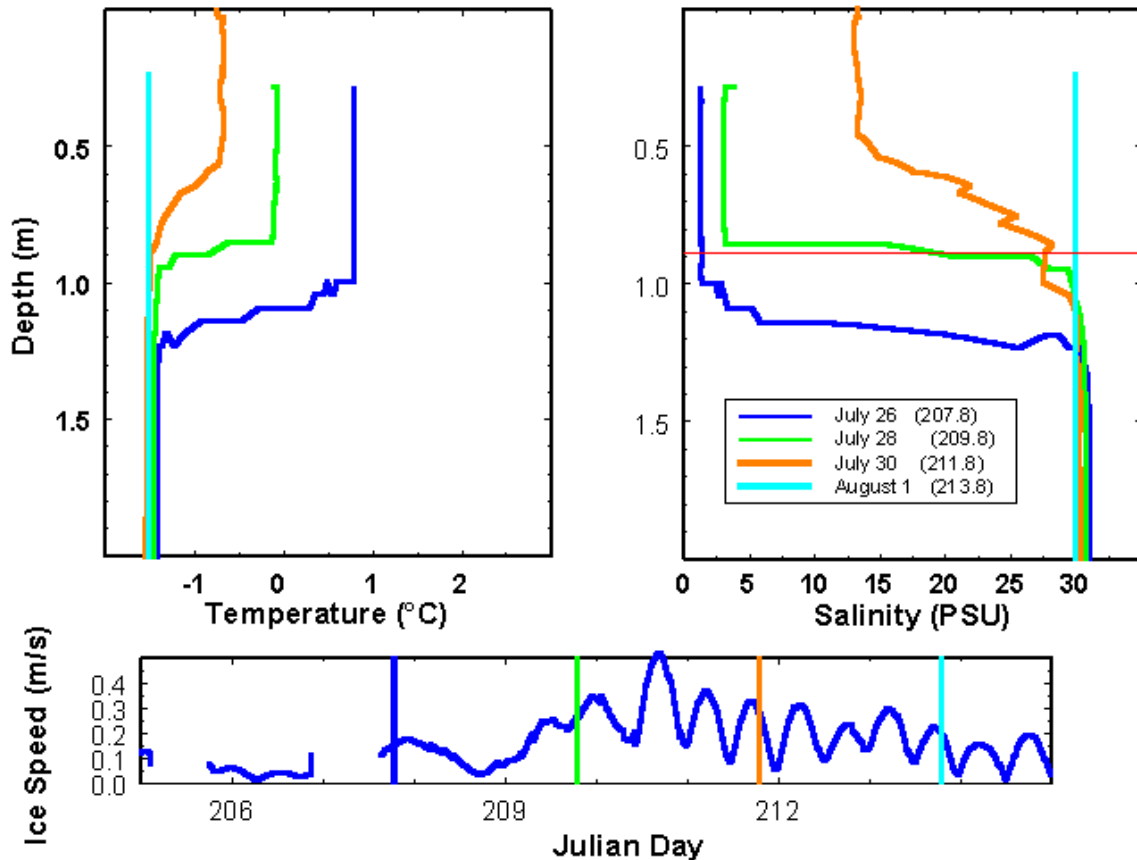
Figure 2. Temperature and salinity profiles in Nanook lead which illustrate the mixing of a fresh, warm, surface layer due to the action of a storm (winds in excess of 10 m/s) in late July. The horizontal line across the right panel shows the depth of surrounding ice floes. The lowest panel (courtesy of M. McPhee) shows ice speed with a maximum of 0.5 m/s associated with the storm. The vertical lines in this panel are at the times of the profiles.
